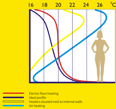
VERTICAL DISTRIBUTION OF TEMPERATURE IN A ROOM FOR THE VARIOUS TYPES OF HEATING
